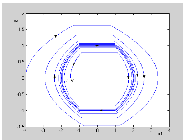
Figure 2.15 Initial condition responses resulting in a limit cycle
